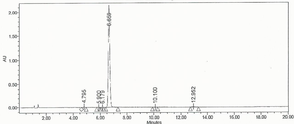
Auto-Scaled Chromatogram
